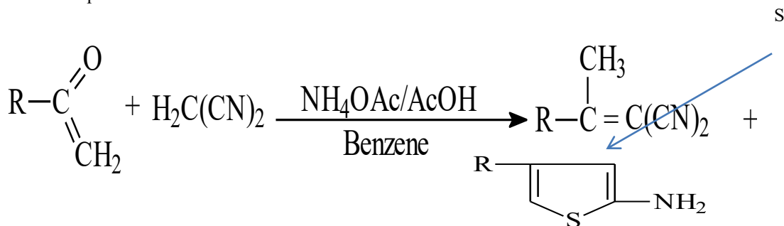
Scheme 1: Gewalds synthesis of aminothiophene derivatives
