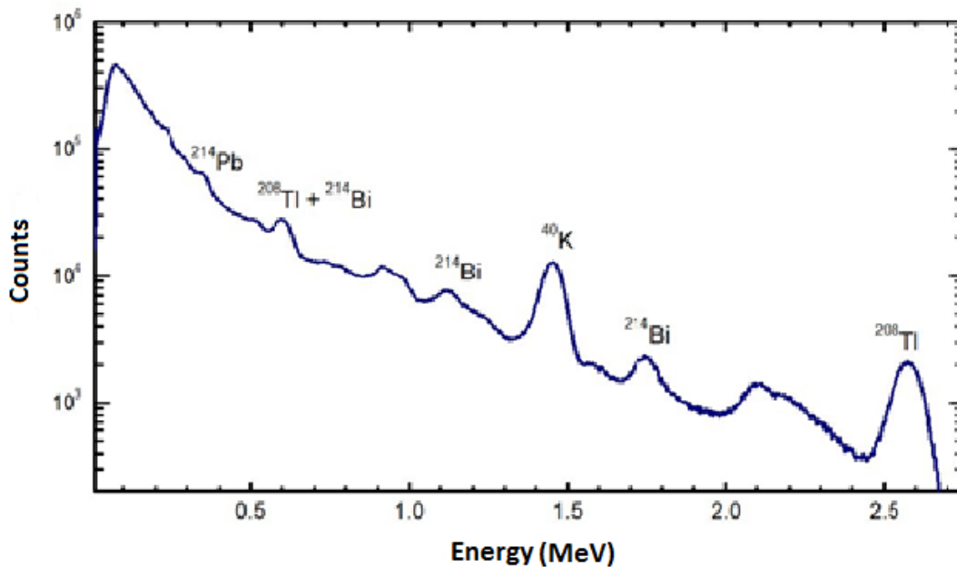
Fig. 8 – Spectrum from 30 keV to 3.0 MeV energy measured in São José dos Campos, SP, during a dry and cumulative time 24 hour period. Energy of some spectral lines photopics: ^{40}\text{K} , (1.46 MeV); ^{208}\text{Tl} , (2.6 MeV); ^{214}\text{Bi} , (0.609 MeV).
