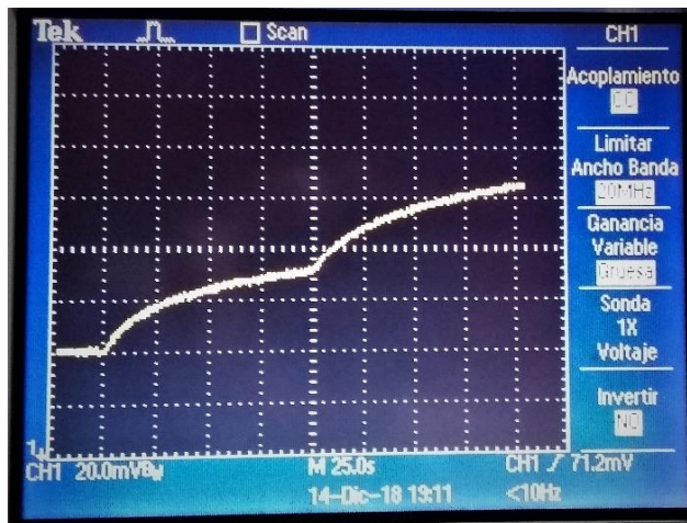
Figure 3: Trace of sensor voltage output, showing the superposition of effects with two emitters irradiating at once
